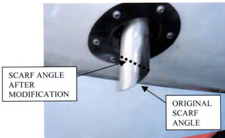
Figure 3: Exhaust Modification
